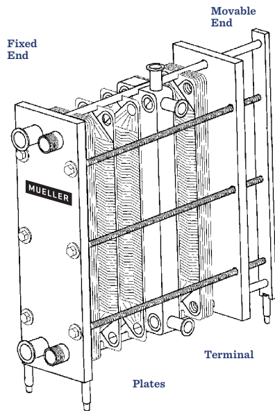
FIGURE 1A - SANITARY FRAME DESIGN
