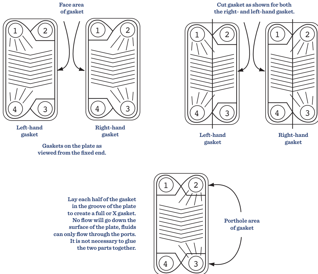
FIGURE 12 - GASKET REPLACEMENT
