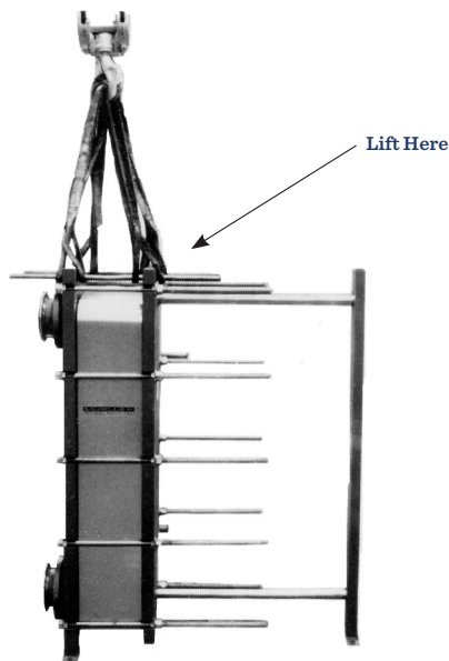
FIGURE 14 - LIFTING INSTRUCTIONS FOR SKID-MOUNTED UNITS
