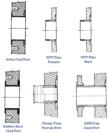
FIGURE 8 - CONNECTION TYPES
