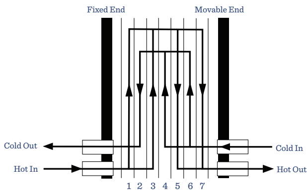
FIGURE 6 - MULTIPLE PASSES
