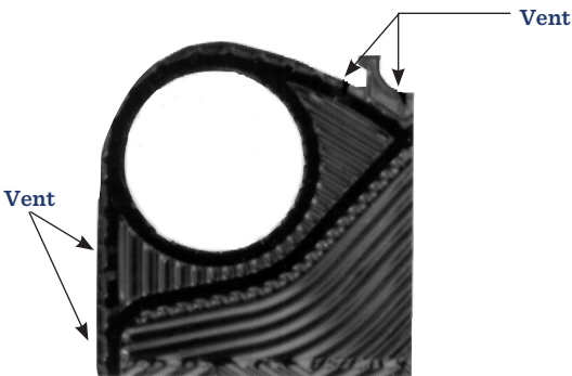
FIGURE 10 - VENT LOCATION
