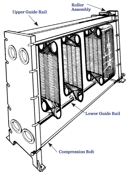
FIGURE 1B - INDUSTRIAL FRAME DESIGN
