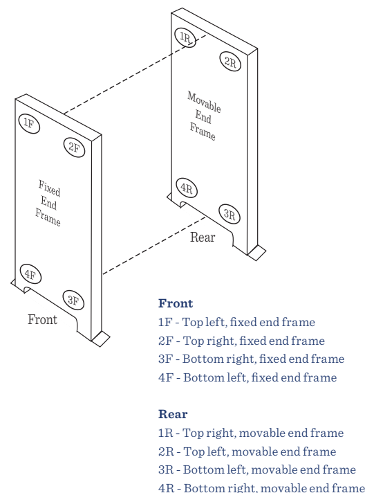
FIGURE 2B - PORT CONFIGURATION
