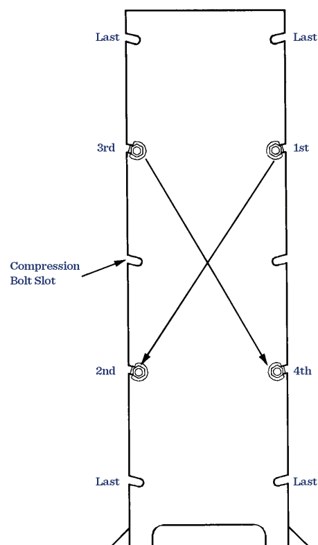
FIGURE 15- PLATE-PACK ASSEMBLY AND TIGHTENING SEQUENCE
