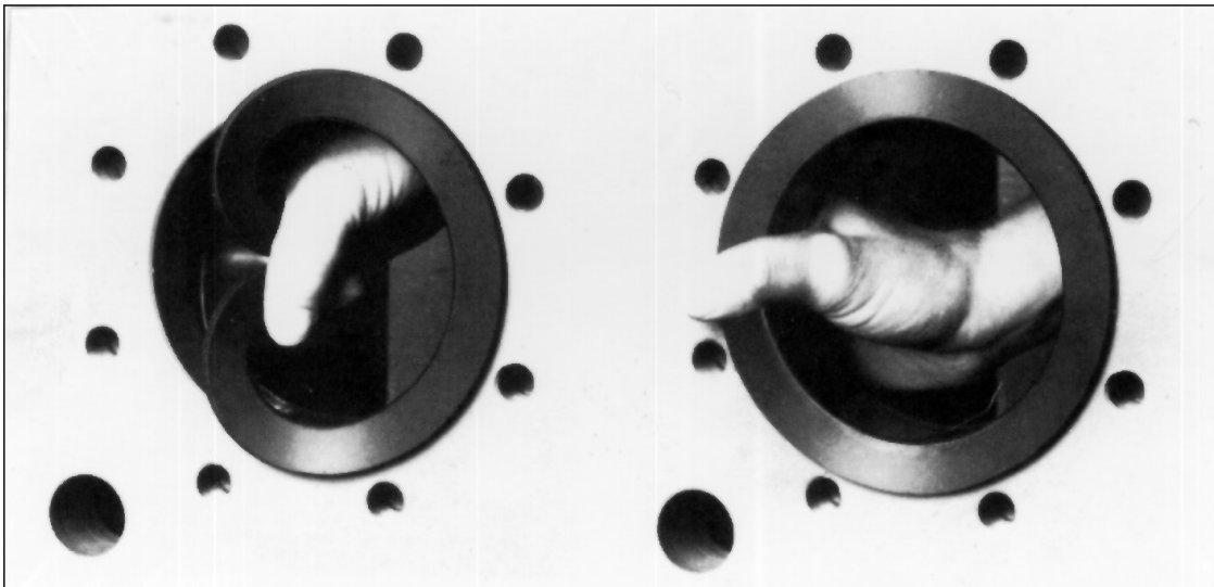
FIGURE 13 - ELASTOMERIC PORT-LINER REPLACEMENT
