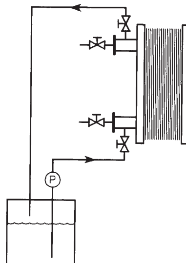
FIGURE 16- CLEANING SOLUTION FLOW
