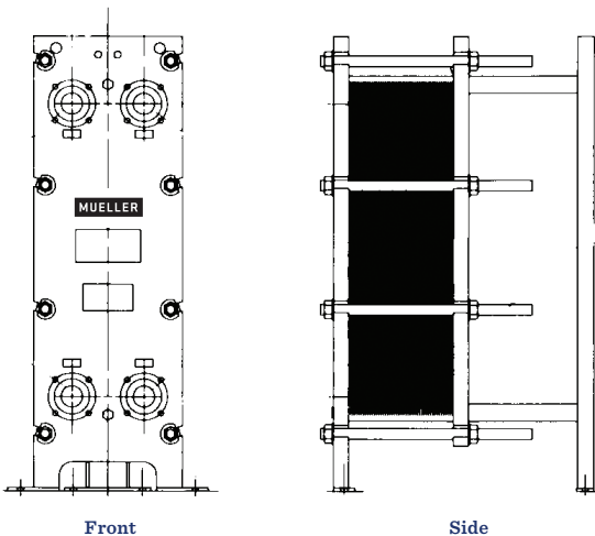
FIGURE 9C - "F" FRAME
