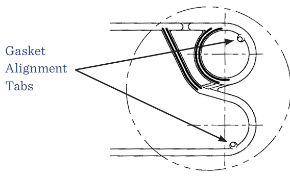
FIGURE 18 - GASKET DETAIL FOR MODEL AT-4
