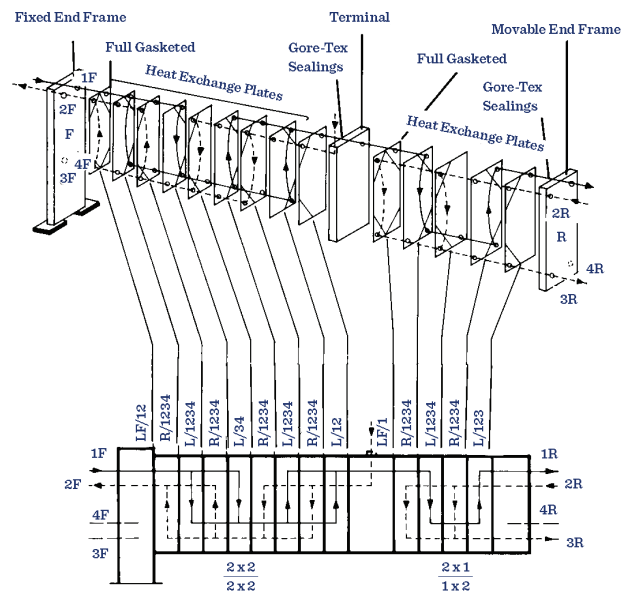
FIGURE 7 - TERMINAL PLATES
