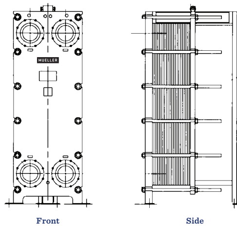
FIGURE 9B - "B" FRAME
