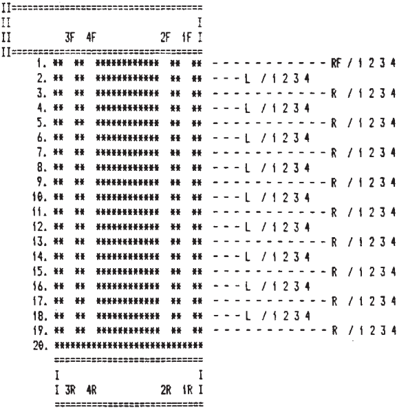
FIGURE 5 - TYPICAL PLATE SEQUENCE AND FLOW DIAGRAM
